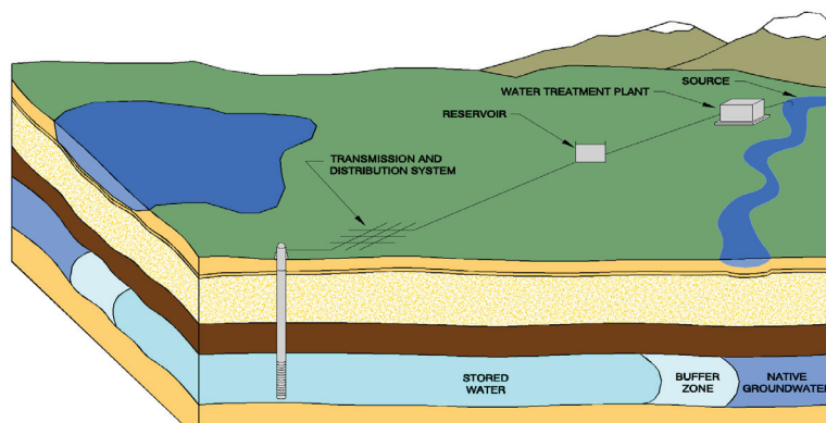
Figure 5: Conceptual ASR Application Illustration. Modified from CH2M HILL.
